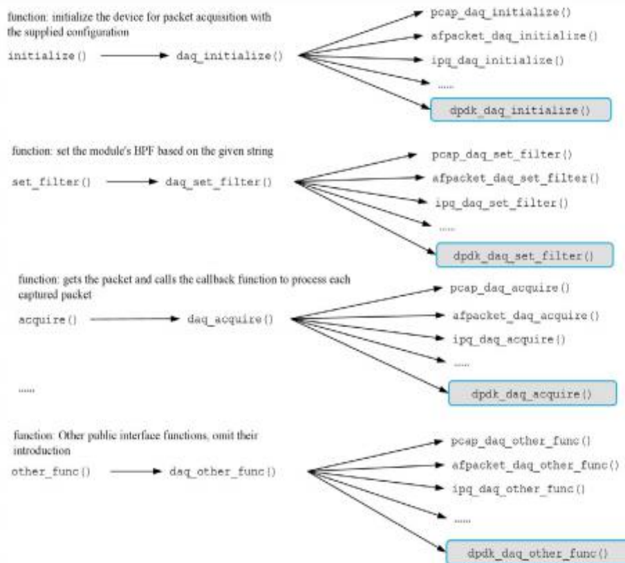
Fig. 3. Snort DAQ common interface function-level
