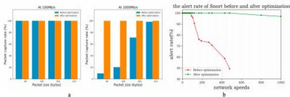
Fig. 4 (a) the packet capture rate at different network speeds before and after optimization; (b) the alert rate of Snort before and after optimization
